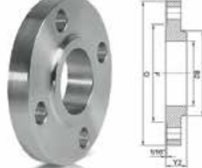
PASLANMAZ 150-300 Lbs SLIP ON FLANŞ
